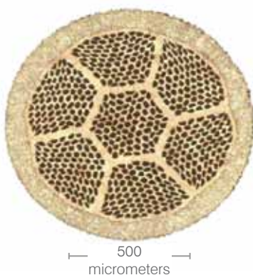
Cross section of a B-2212 HTS filamentary wire (Courtesy of Oxford Instruments)
