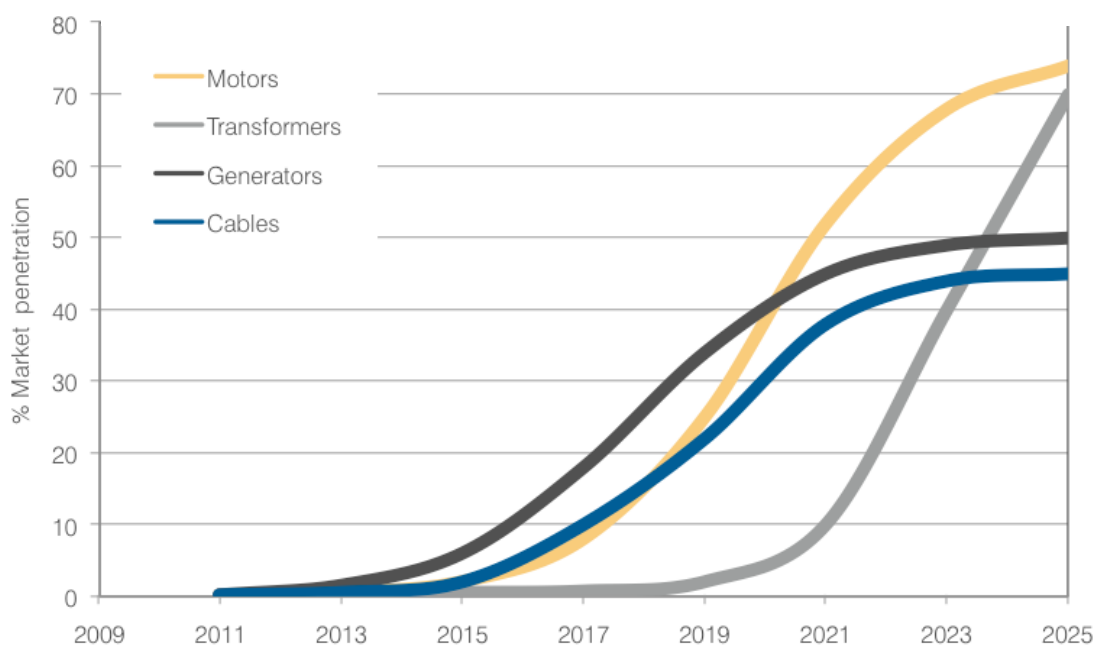
Figure 19: Predicted market penetration curves - HTS power devices
