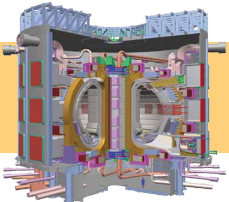
Figure 11: ITER machine mass: 23350 t (cryostat + VV + magnets) – Shielding, divertor and manifolds: 7945 t + 1060 port plugs – magnet systems: 10150 t; cryostat: 820 t. Courtesy of ITER publications.
